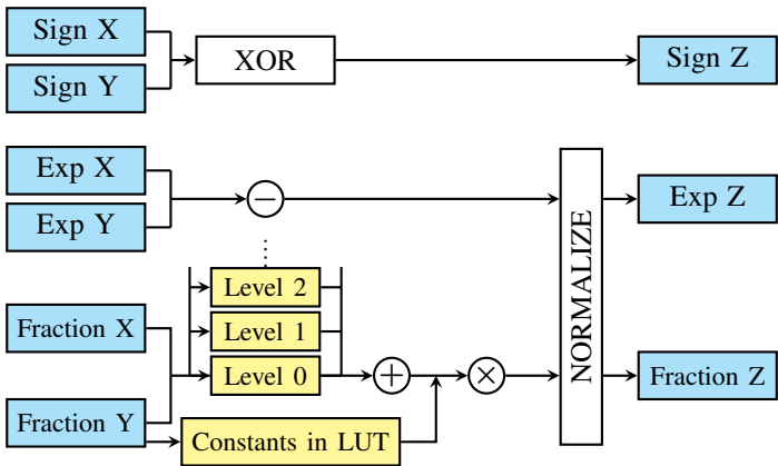
Fig. 1. Architecture of the proposed approximate divider.
